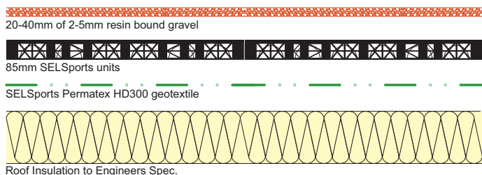
Typical Resin Bound Gravel Construction
