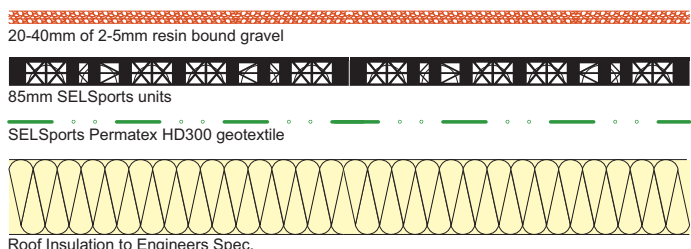
Typical Resin Bound Gravel Construction
